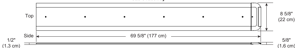
Cable raceway
